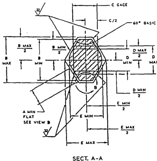
SECT. A-A
